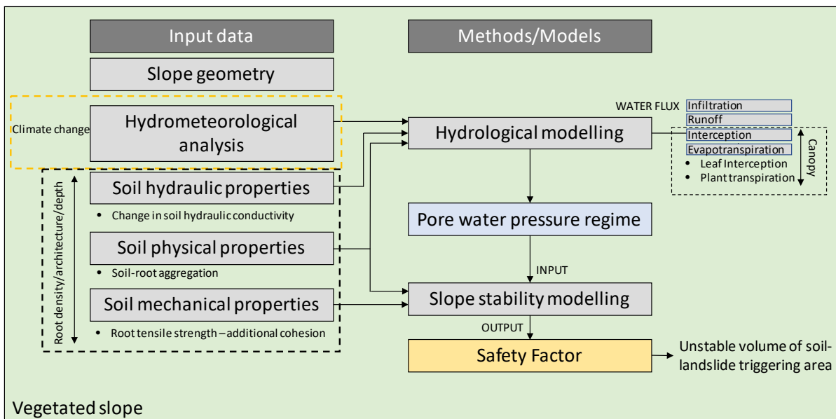
Figure 1 Methodological approach for slope stability modelling including vegetation– soil parameters and processes influenced by the presence of vegetation (root density/architecture/depth and canopy area).
