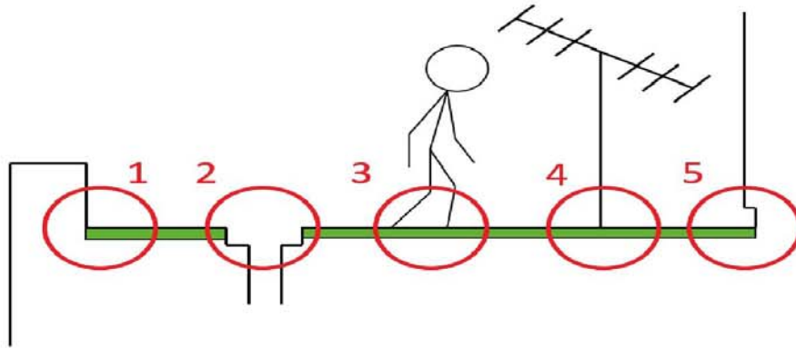
Figure 16: Critical vulnerable points of a green roof (also applicable for blue-green roofs): 1) Transitions between the roof and parapets. 2) Drains. 3) Traffic or work on the roof, including the use of tools such as landscaping tools or ladders. 4) Fastening points for technical equipment that perforates the roofing membrane. 5) Transitions between the roof and walls, particularly around doors.
